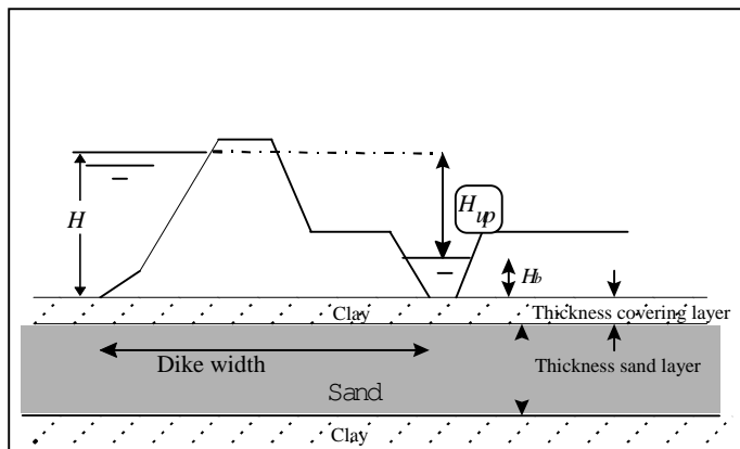
Figure 1. Cross-section of a dike.
