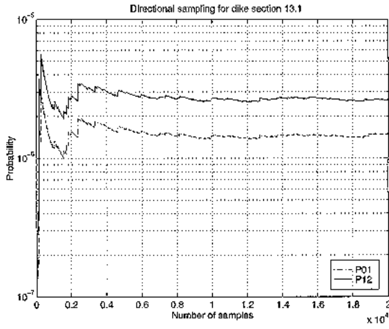
Figure 2. The probability of failure of one subsection ('P01') and two subsections ('P12') of dike section 13.1 determined on the basis of 20,000 samples using three-dimensional directional sampling.
