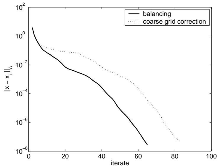
Figure 2: Convergence of the balancing and additive coarse grid correction preconditioner with \gamma = 500 and x_0 = ZE^{-1}Z^T r_0 .
