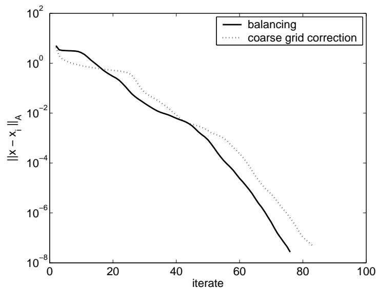
Figure 3: Convergence of the balancing and additive coarse grid correction preconditioner with \gamma = 500 . In this example a random starting vector is used.
