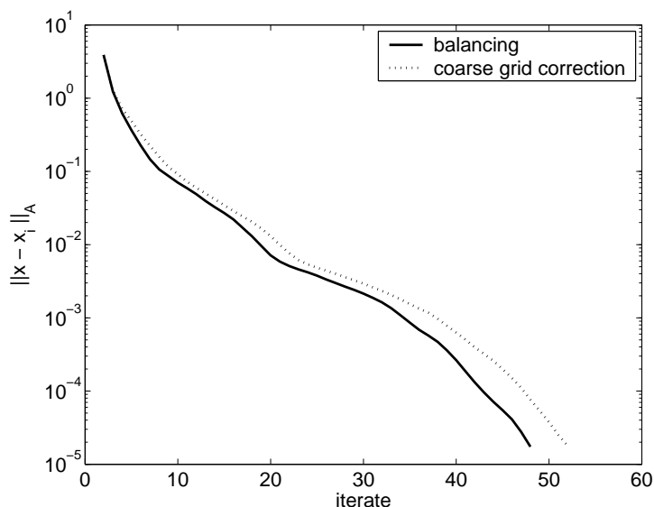
Figure 1: Convergence of the balancing and additive coarse grid correction preconditioner with \gamma = 1 and x_0 = ZE^{-1}Z^T r_0 .
