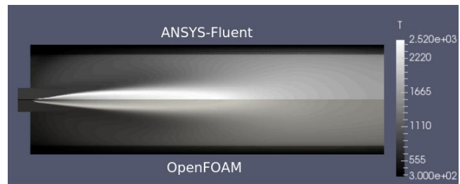
Figure 7: Comparison of the contour plots of the temperature (K) in Case 3 (radiation switched off).
