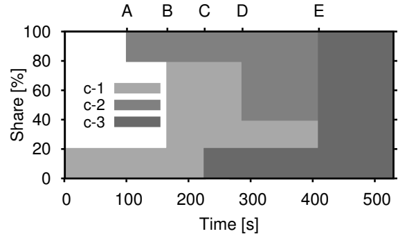
Figure 6: The distribution of the resources across three MR-clusters (c-1, c-2, c-3) arriving at different moments in time. (Points A-E explained in Section 7.1.)
